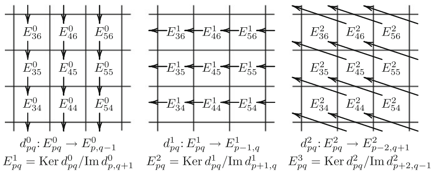
Fig. 75 Diagrams for the terms E^0, E^1, E^2 of a spectral sequence
