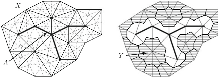
Fig. 71 A barycentric star complex approximation of X - A
