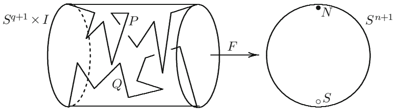
Fig. 55 Proof of the monomorphism part of Freudenthal's theorem
