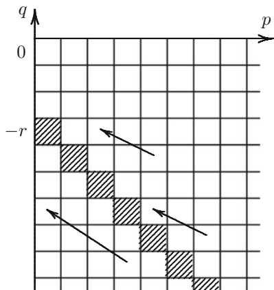
Fig. 134 The Atiyah–Hirzebruch spectral sequence for \Pi
