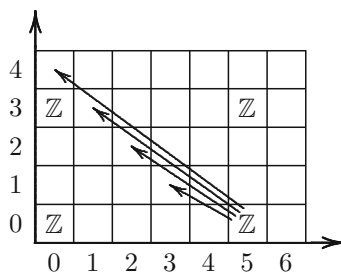
Fig. 81 The E^2 -term for the fibration SU(3) \xrightarrow{S^3} S^5
